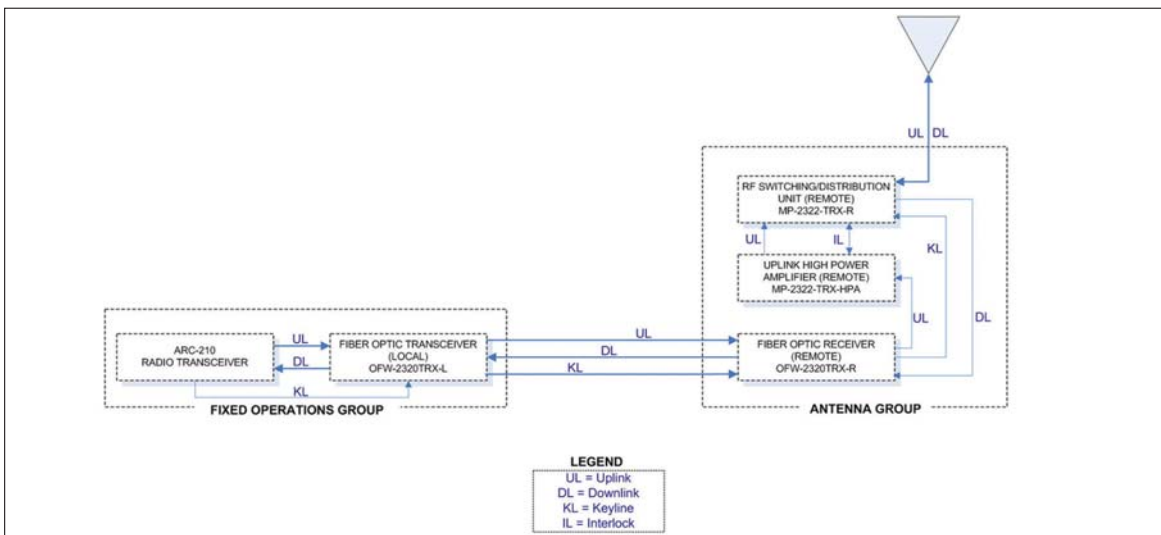
Tactical Radio Deployment - Function Block Diagram
